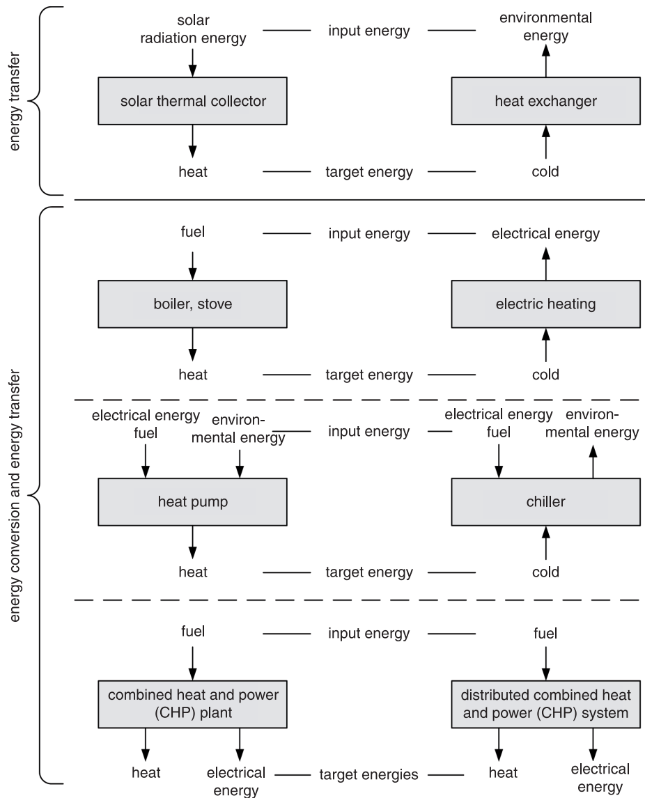
Figure 1. Overview of possibilities of heat and cold “generation” through energy conversion and energy transfer [1]
